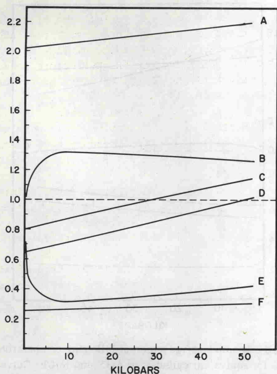
Fig. 14 Labeled curves represent following comparative ratios for equivalent cylinders of AgCl and MgO: Curve A = Poisson's ratios according to AgCl/MgO. Curve C = Young's moduli according to AgCl/MgO. Curve D = moduli of rigidity according to AgCl/MgO. Curve E = radial displacement, U_R , according to MgO/AgCl. Curve F = moduli of compression according to AgCl/MgO. Curve B = ratio P_i/P_e for case of a solid cylindrical core of MgO enclosed by a cylindrical shell of AgCl which is subjected to an external hydrostatic pressure, P_e
