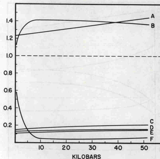
Fig. 15 Labeled curves represent following comparative ratios for equivalent cylinders of MgO and NaCl: Curve A = Poisson's ratios according to NaCl/MgO. Curve C = moduli of compression according to NaCl/MgO. Curve D = Young's moduli according to NaCl/MgO. Curve E = moduli of rigidity according to NaCl/MgO. Curve F = radial displacement, U_R , according to MgO/NaCl. Curve B = ratio P_i/P_e for case of a MgO solid cylindrical core enclosed by a NaCl cylindrical shell subjected to an external hydrostatic pressure, P_e
