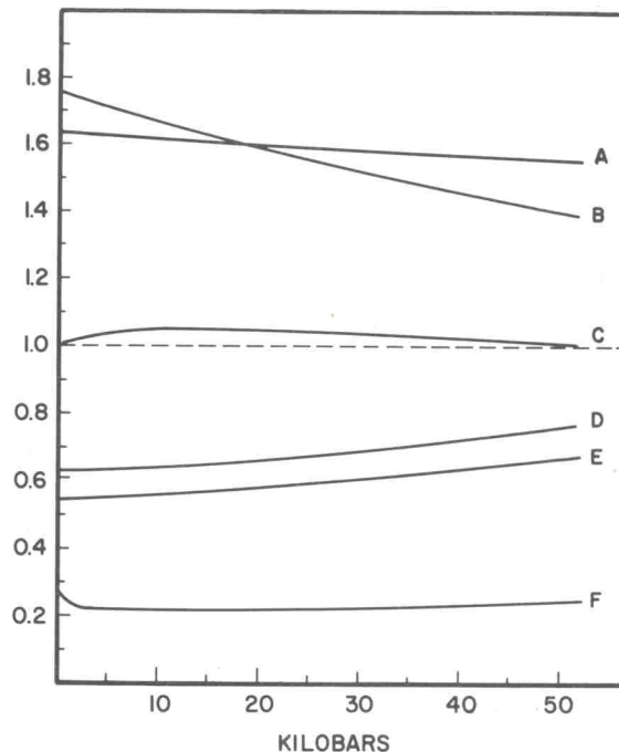
Fig. 13 Labeled curves represent following comparative ratios for equivalent cylinders of AgCl and NaCl: Curve A = Poisson's ratios according to AgCl/NaCl. Curve B = moduli of compression according to AgCl/NaCl. Curve D = Young's moduli according to AgCl/NaCl. Curve E = moduli of rigidity according to AgCl/NaCl. Curve F = radial displacement, U_R , according to NaCl/AgCl. Curve C = ratio P_i/P_e for case of a solid cylindrical core of NaCl enclosed by a cylindrical shell of AgCl which is subjected to an external hydrostatic pressure, P_e
